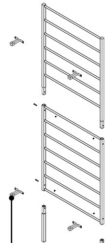
84" H Industrial Steel Tube Ladder Trellis
