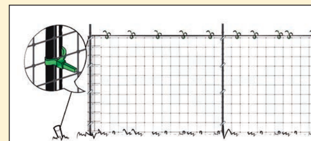
INSTALLATION WITH METAL T POST
