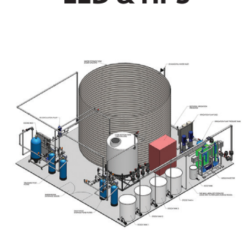
Water Treatment
