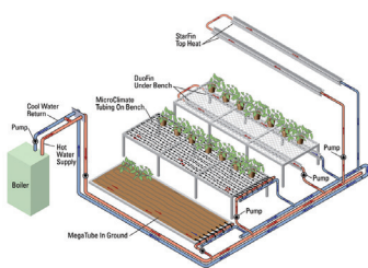
Heating & Cooling
