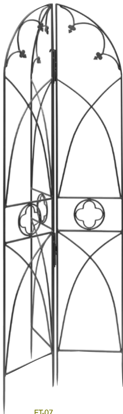
FT-07 Quatrefoil Trellis Each Panel: 13"W x 75"H Consists of 3 sections Opened: 22" - 26"W Graphite
