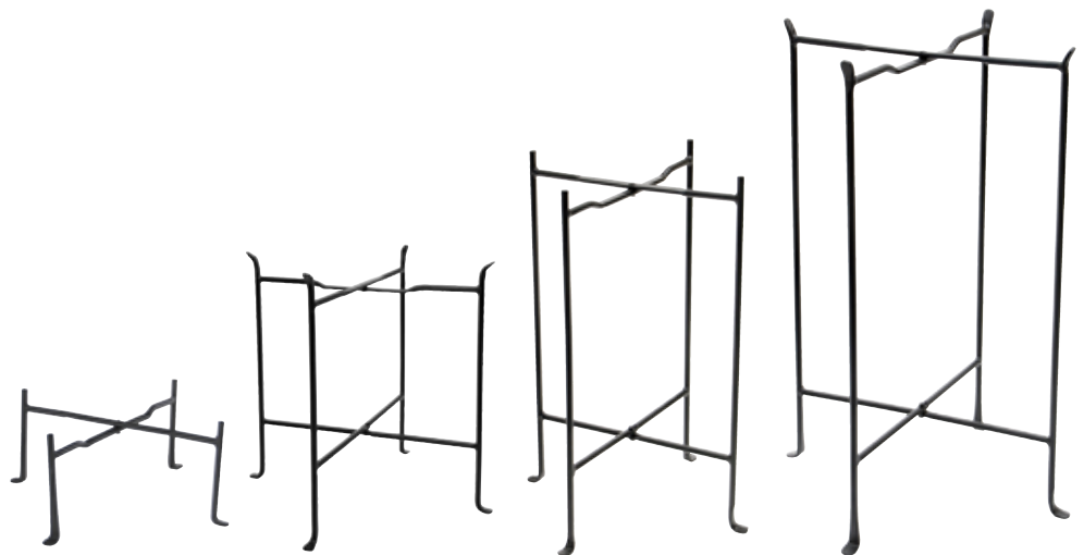
CWI-04 Short Floor 19½" H x 15" sq. opened 20½" L x 2¾" D closed Shelf: 18" L x 2" D
